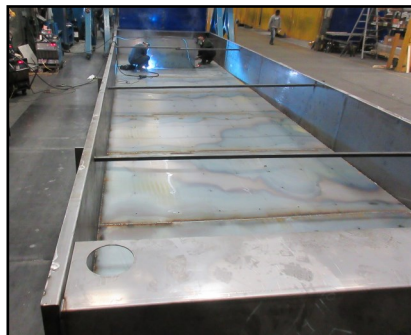
From left: Tramont engineers work on a tank design. 9000-gallon Sub Base Tank under construction. Final inspection of Sound-Attenuated Enclosure Package.
